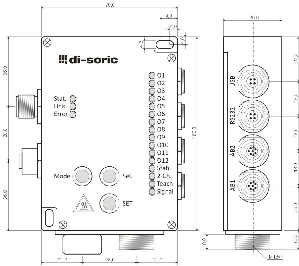
Figure 4 : Drawings FS 12-100-1 M G8-B8-PB with built-in control devices for the drift stabilization CROMLASTAB®
