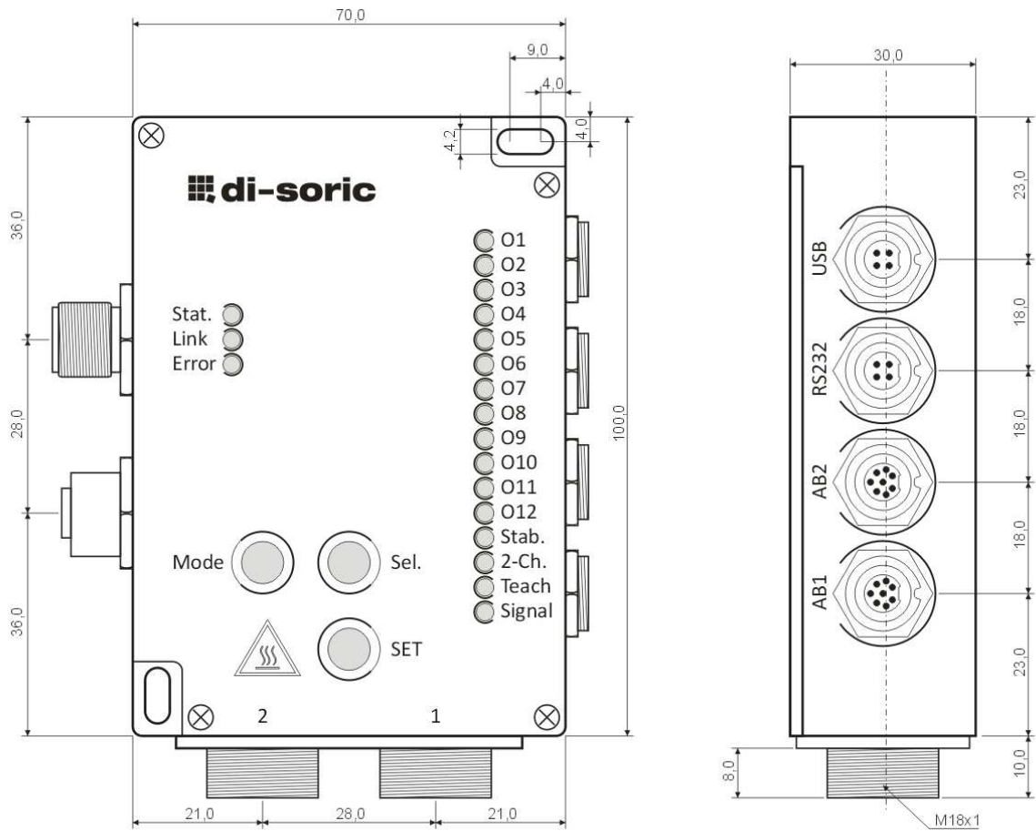
Figure 3 : Drawings FS 12-100-2 M G8-B8-PB for connecting two separate fiber optical cables
